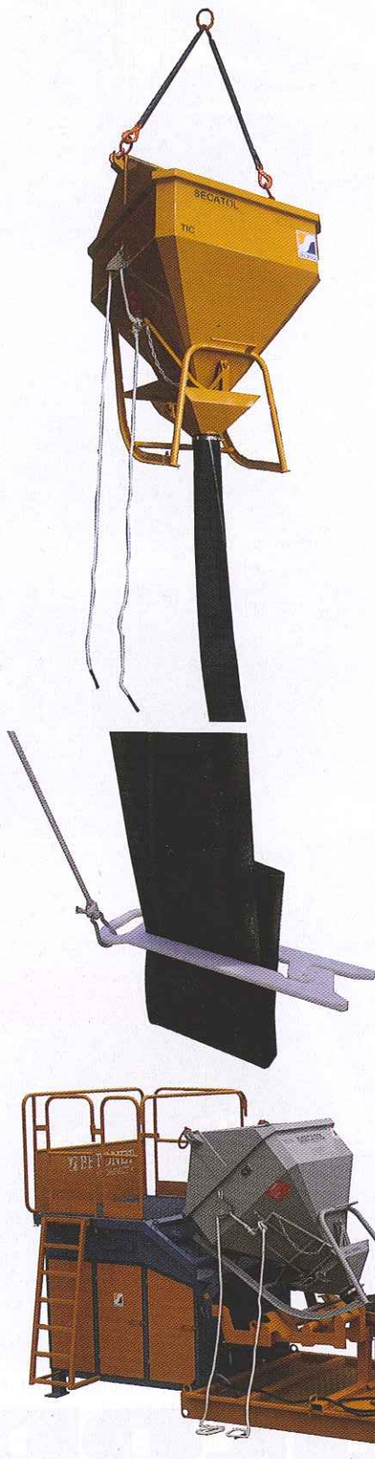
TIC PF concrete skip with auto-locking hose clip and Betonet washing platform
